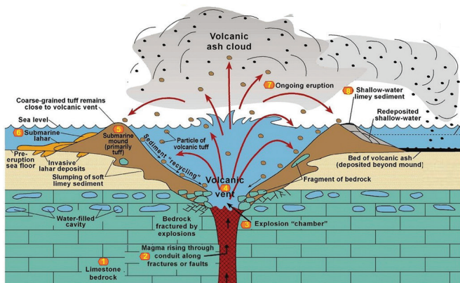
Figure 2. Schematic model of an erupting submarine volcano (modified from Caran et al. [2012] and Ewing and Caran [1982]). The construction of a tuff mound began with a “phreato magmatic” (steam + magma) eruption. Magma rising along a dike feeder met abundant water either at the seafloor or in a porous, water-saturated unit at moderate depth beneath the seafloor (Ewing and Caran [1982] and Caran et al. [2012]).
