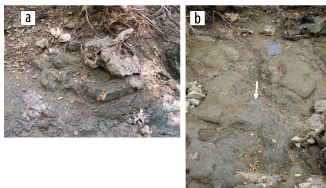
Figure 5. (a) Pillow lava and (b) lava tube structure on the bed of Williamson Creek. The arrow in 5b shows the direction of lava flow. (Photos courtesy of Alan Cherepon and Chris Caran, respectively).
