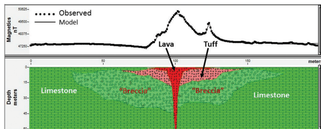
Figure 11. Forward model of magnetic profile MR. To have a good fit, very high (red), high (pink), and low (light green, breccia) magnetic zones were assumed. The magnetic susceptibility of the country rock (limestone) was taken zero (see text for detail). The width of the volcanic vent is about 17 m near the surface, but it decreases with depth.
