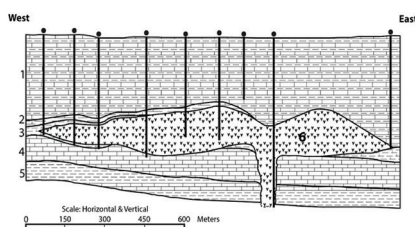
Figure 3. (Taken from Sellards [1932] and modified for simplicity.) West-east cross section of Chapman oil field showing relation of serpentine mass to overlying and underlying formations. (1) Taylor and overlying younger formations; (2) Taylor; (3) chalk stratum near base of Taylor; (4) Austin Chalk; (6) serpentine. Locations of nine oil wells (black dots) are shown along the cross section, seven of which are in the serpentine plug. The width of the eruption center is about 60 m.
