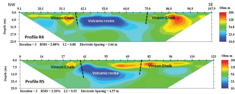
Figure 9. Resistivity data along profiles R4 and R5 on the southern bank of Williamson Creek. Geologic contacts (dashed black lines) observed on the bed of the creek extended and projected on the resistivity data. High magnetic values on profiles M3 and M4 (~48,500 and 47800 nT, respectively), which are located near these resistivity profiles, correspond to the low-resistivity anomalies, as depicted with the blue color.
