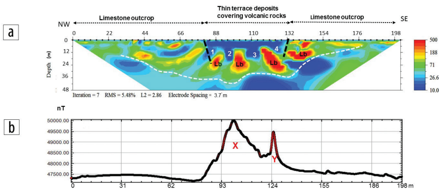
Figure 10. (a) Resistivity and (b) magnetic data along profile MR on the south bank of Williamson Creek. High resistive, fragmented limestone blocks (Lb) underlie the low-resistive volcanic rocks. Note the interfingering geometry of the volcanic rocks, shown with numbers 1, 2, 3, and 4. Locations of contacts (dashed-black lines) are precisely shown on the resistivity map because they were observable on the bed of the creek. The width of the volcanic section is approximately 50 m. The magnetic data indicates two high anomalies, shown with letters X and Y.
